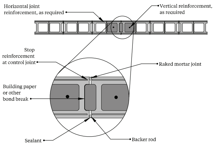
Figure 7d - Formed paper joint (4-hour fire rated)
