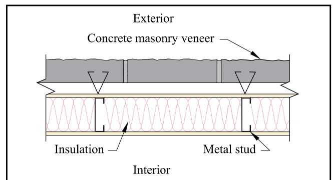
Figure 2—Concrete Masonry Veneer with Steel Stud Backup
