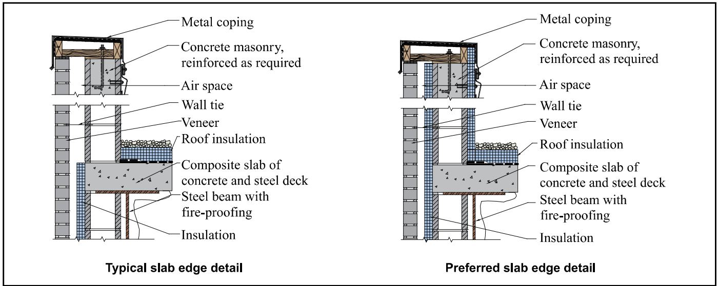
Figure 4—Alternative Insulation Strategies for a Masonry Parapet
