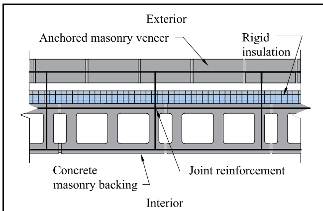
Figure 1—Insulated Masonry Cavity Wall
