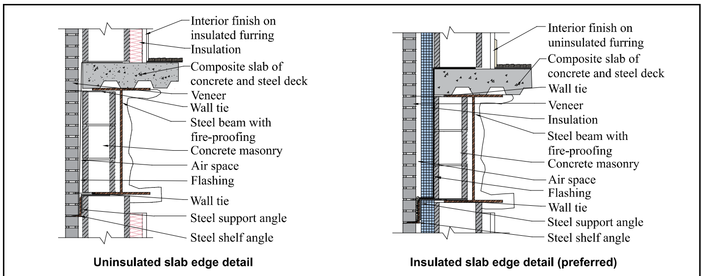
Figure 3—Alternative Insulation Strategies for Slab Edge and Perimeter Beam
